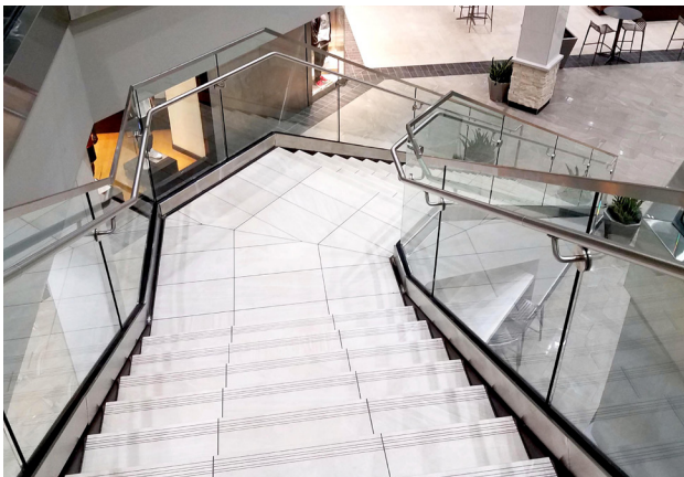
Clear half-inch glass is secured within an aluminum shoe using Trex Commercial Products' dry glaze GlassNut™ Track Rail system, with a black gasket finishing off the look.
